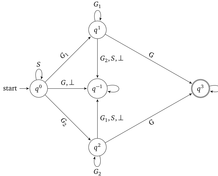
Fig. 3. The DFA for the second task of the case study.
