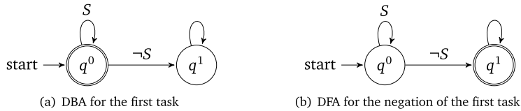
Fig. 2. Automata representation of the first task of the case study in Section 2.2.
