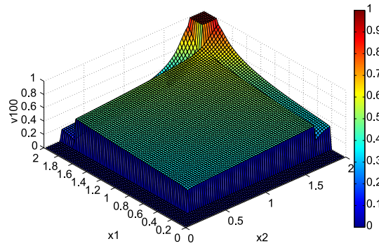
(a) DFA value function plotted in 3d
